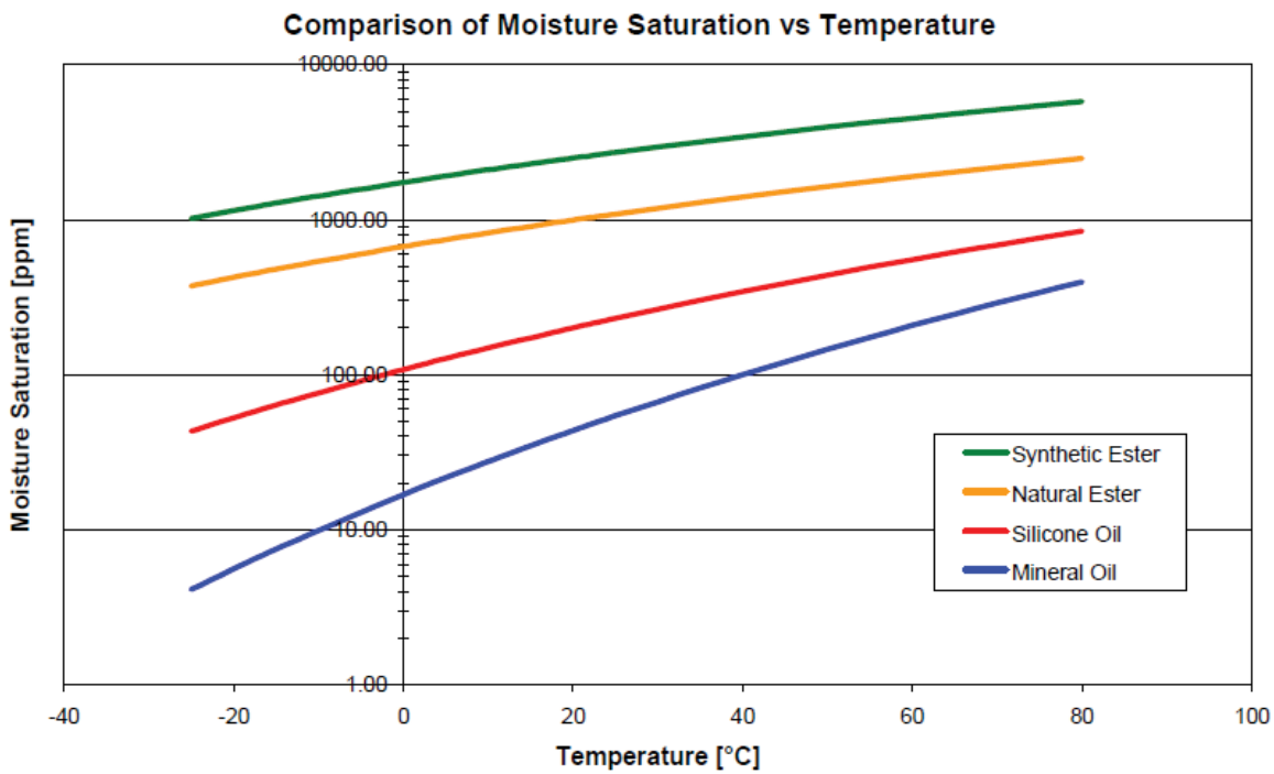
Courtesy : CIGRE 436 - Experiences in service with new insulating liquids Figure 1.0 - How moisture saturation varies with temperature
