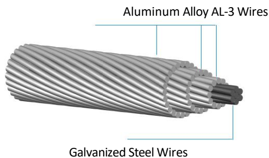
Fig. 1 AACSR Conductor
