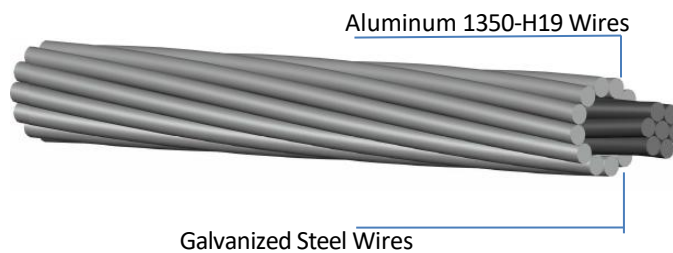
Fig. 1 ACSR Dotterel Conductor
